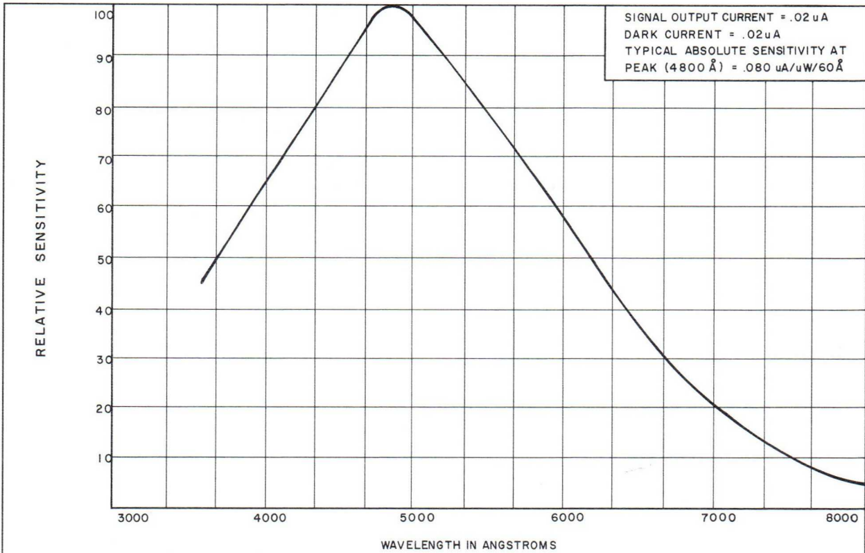
FIG. 4 SPECTRAL RESPONSE
