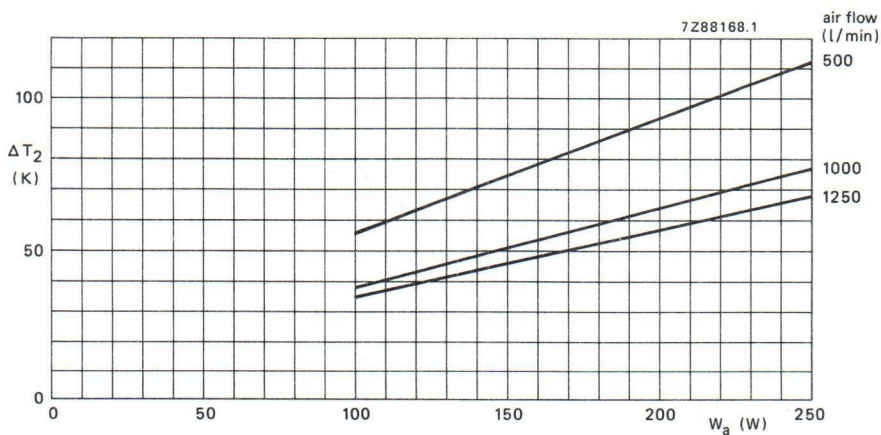
Fig. 6 Increase of anode temperature above inlet air temperature, \Delta T_2 , as a function of anode dissipation, W_a . Anode dissipation = (peak anode voltage) \times (average anode current) - (output power). V_f = 3,4 V.
