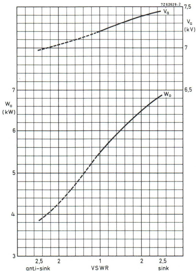
Fig. 15 Output power and anode voltage as a function of load impedance, V_f = 1,0 \text{ V} ; I_{a \text{ mean}} = 1,25 \text{ A} .
