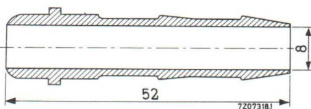
Fig. 6 9 mm hose nipple type TE 1051c.
