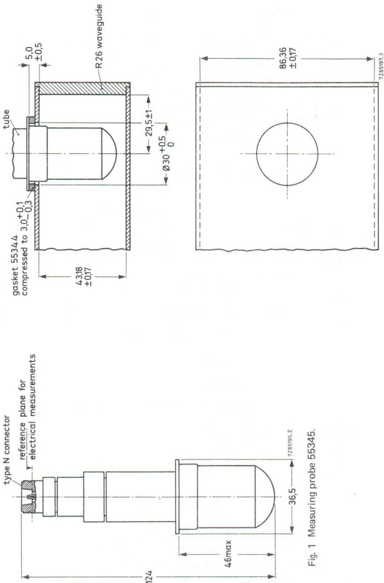
Fig. 1 Measuring probe 55345.
