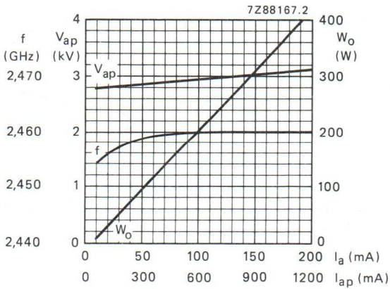
Fig. 8 Performance chart 2.
