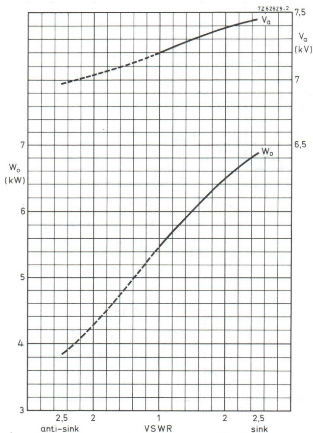
Fig. 15 Output power and anode voltage as a function of load impedance, V_f = 1,0 V; I_{a \text{ mean}} = 1,25 A.
