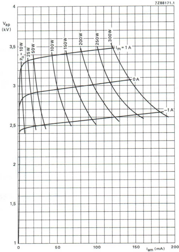
Fig. 2 Performance chart 1.
