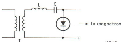
Fig. 2 Basic circuit of an LC stabilized half-wave doubler anode supply unit.
