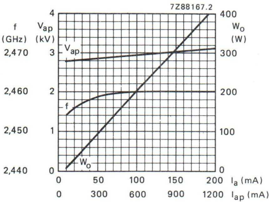
Fig. 7 Performance chart. f = f(I_{ap}) ; V_{ap} = f(I_{ap}) ; W_o = f(I_a) .
