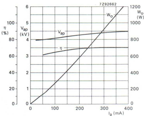
Fig. 6 Performance chart.
