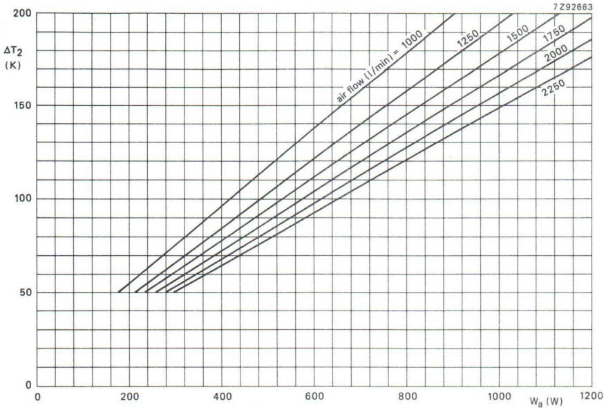
Fig. 5 Increase of anode temperature above inlet air temperature, \Delta T_2 , as a function of anode dissipation, W_a . Anode dissipation = (peak anode voltage) x (average anode current) – (output power).
