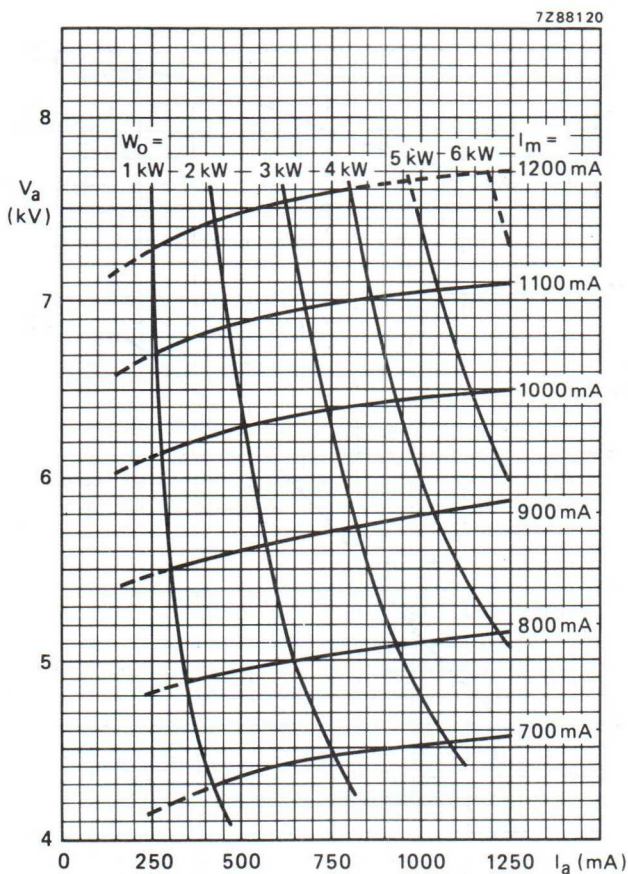
Fig. 14 Performance for VSWR = 1,5 in the phase of sink direction. Output power and anode voltage as a function of anode current. Anode voltage is a function of the electric current through the magnetic coils ( I_m ). Measured with: Cooling constant; V_f adapted to the output power.
