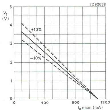
Fig. 3 Filament voltage reduction curve with applied anode voltage. Filament starting voltage without anode voltage is 5,0 \text{ V} \pm 10\% .
