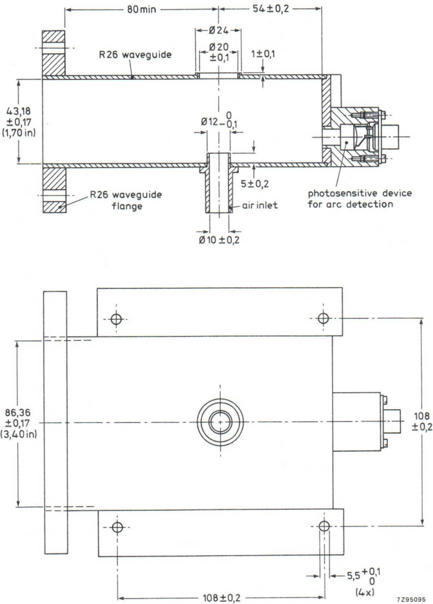
Fig. 6 Waveguide assembly.
