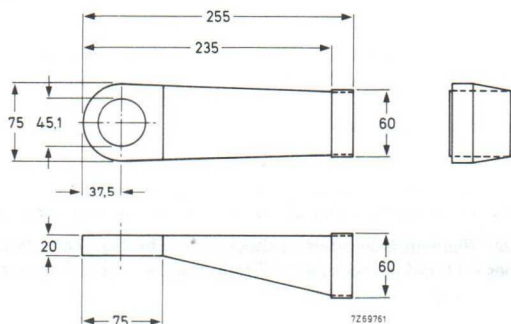
Fig. 8 Cooling device.
