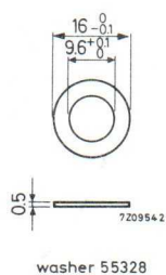
washer 55328
