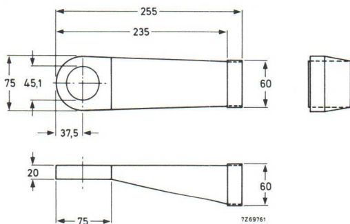
Fig. 8 Cooling device.
