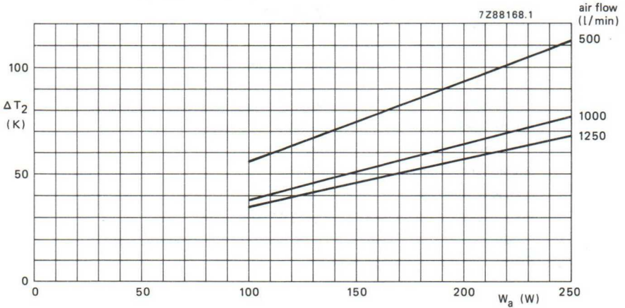
Fig. 5 Increase of anode temperature above inlet air temperature, \Delta T_2 , as a function of anode dissipation, W_a . Anode dissipation = (peak anode voltage) \times (average anode current) - (output power). V_f = 3,4 V.
