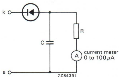
Fig. 3 For 50 Hz operation the RC time is fixed to 1 s.
