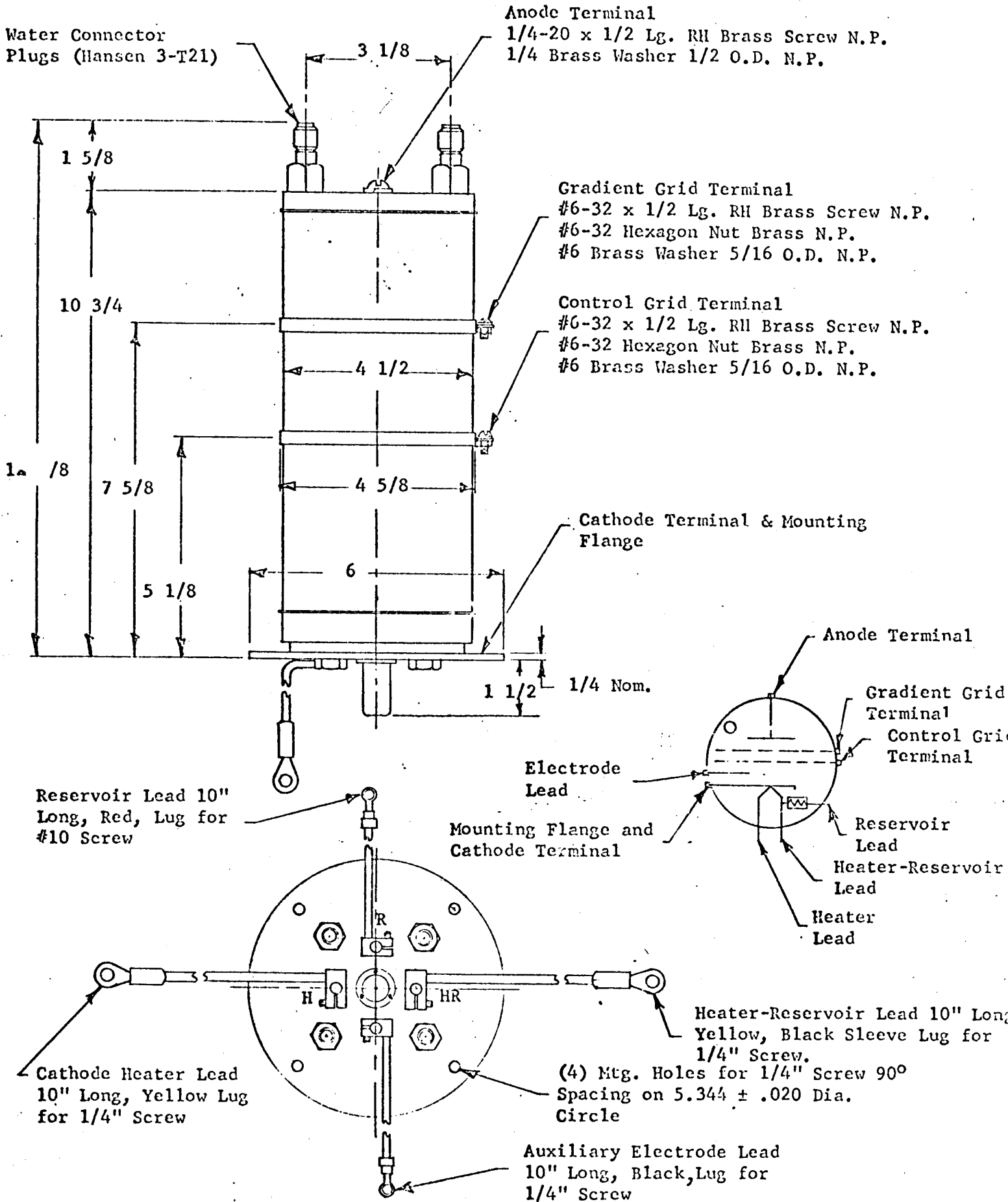
F-104 OUTLINE
